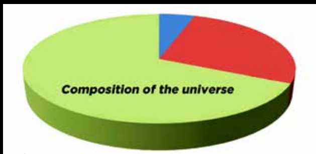
Image 2: Composition of the universe: Blue: matter visible for people Red: undiscovered elementary particles Green: ZPE-energy (according to E=mc^2 ) And the green part of the universe can be utilised as energy!
