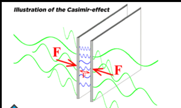
Image 1: The zero-point waves (green) are everywhere in the space, they fulfil the complete universe. But the metallic plates as shown in the picture, exclude some of the ZPE-waves (blue). Due to the fact that each single wave exposes a pressure to the plates, the missing waves in the intermediate space between the plates, leads to a missing pressure even there, so that the ZPE-waves from outside have a higher pressure than the ZPE-waves from inside. The consequence is a force "F", which moves the plates towards each other - an invisible force coming from the quantum vacuum, the namely Casimir-force.
